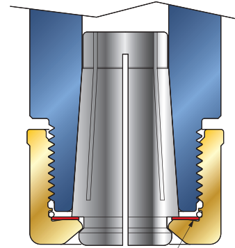
Flat bearing 軸承墊片
